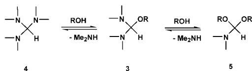
Scheme 2. The Bredereck equilibria.
