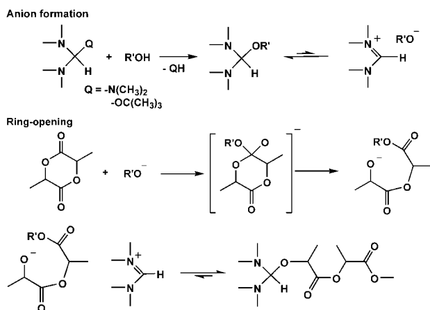
Scheme 4. Proposed mechanism for ROP by 3 and 4 .
