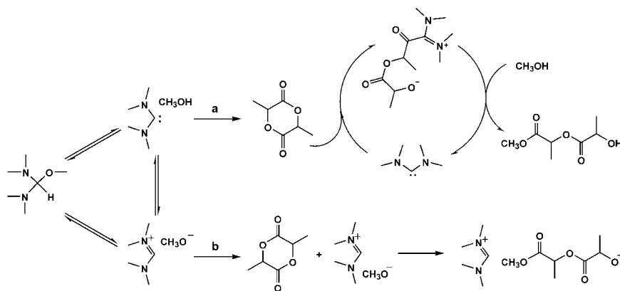
Scheme 3. Possible pathways for ring-opening polymerization by 3b .
