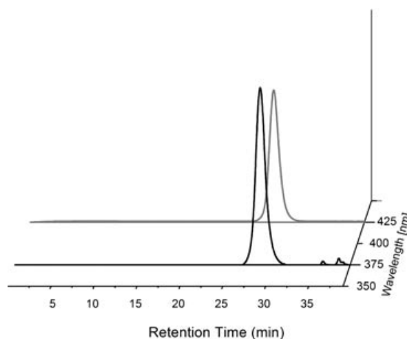
Figure 2. GPC trace of polylactide initiated from 1-pyrenebutanol.
