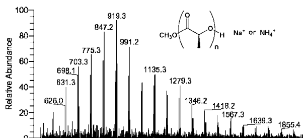
Figure 3. +ESI mass spectrum of oligolactide.
