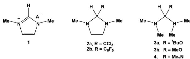
Scheme 1. Potential precursors to N -heterocyclic carbenes.
