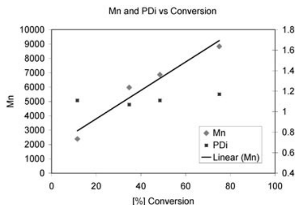
Figure 1. Plot of M_n and PDI versus conversion.
